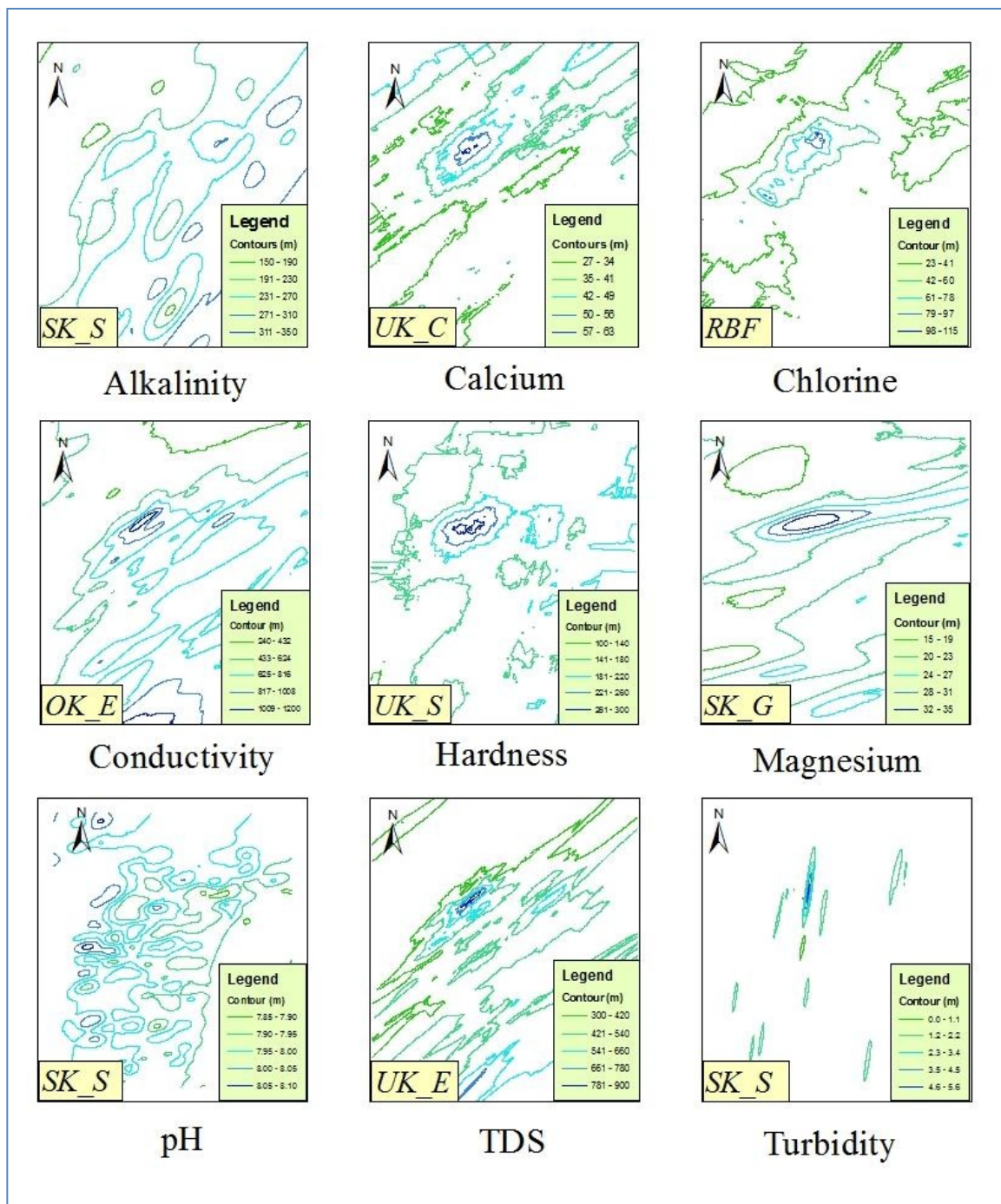
Figure 10: Contour Analysis of Different Water Quality Parameters
