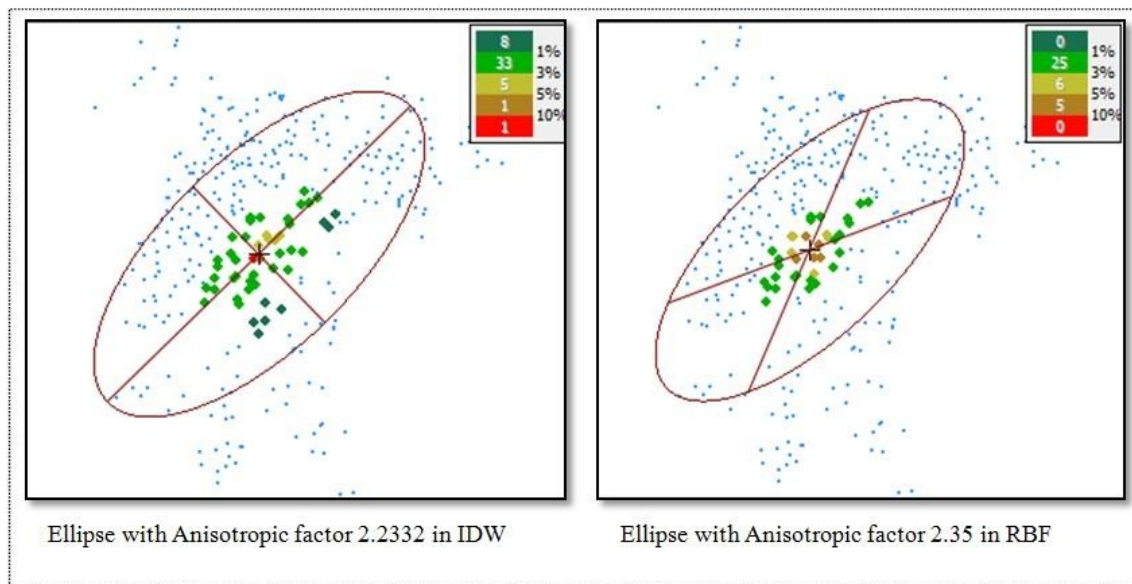
Figure 3: Directional Distribution of Ellipse for Ca
