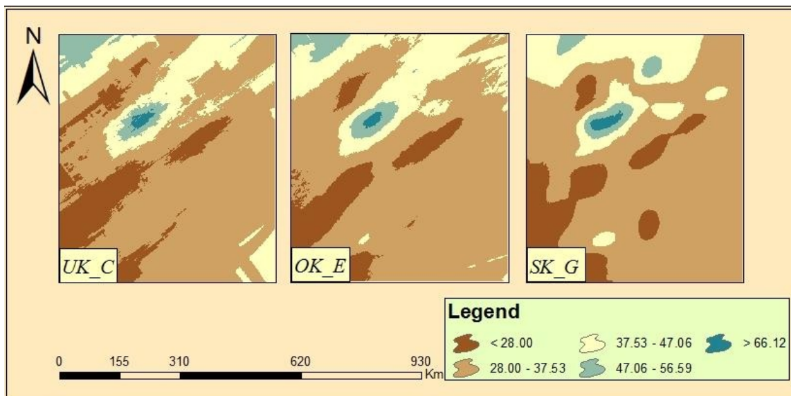
Figure 11: Comparison of Stochastic Methods for Ca
