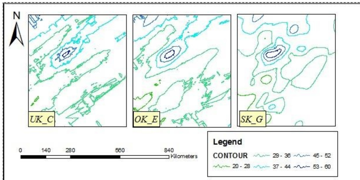
Figure 9: Comparison of Stochastic Methods for Ca
