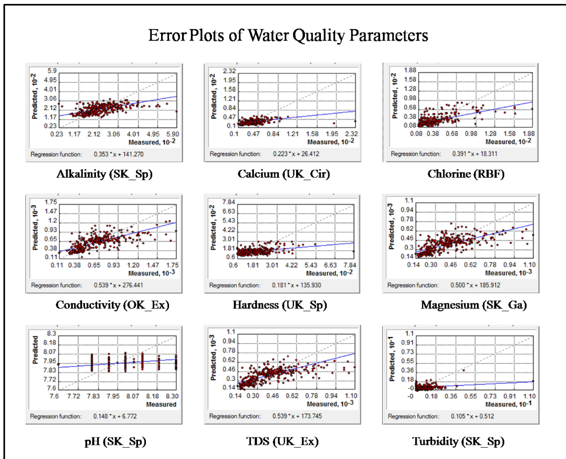
Figure 6: Error Plots of Water Quality Parameters
