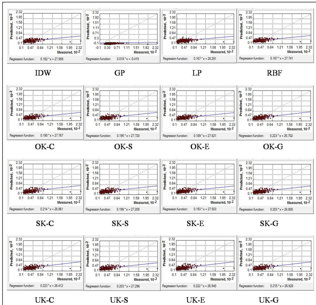
Figure 5: Error Plots of Ca
