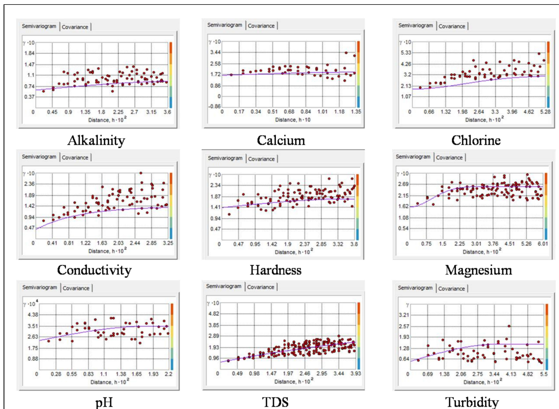
Figure 8: Best Semivariogram of Quality Parameters
