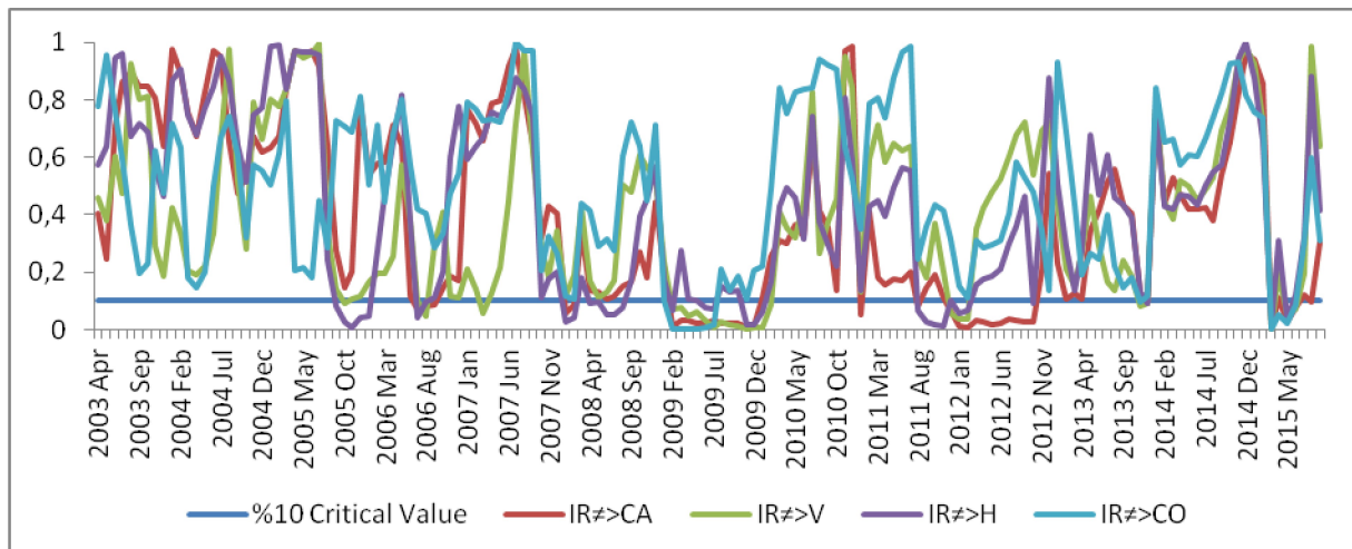
Graphic 1: Results for Balçılar et. al. (2010) rolling window regression causality test
